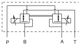
型号 3DREP-02C
